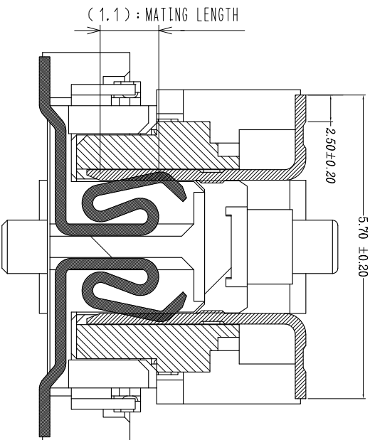
CROSS CUT SECTION (5:1)
