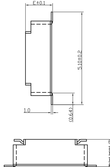
MATING SECTION
