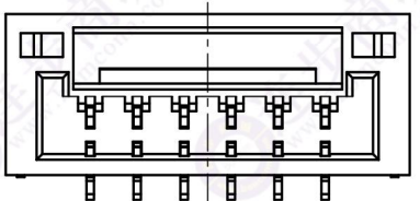
2~6 Pin
