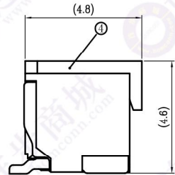
WITH COVER
