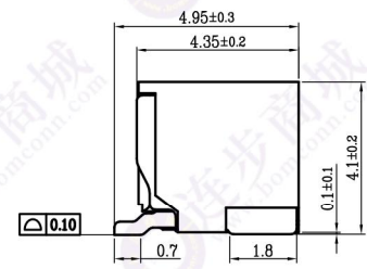
WITH COVER
