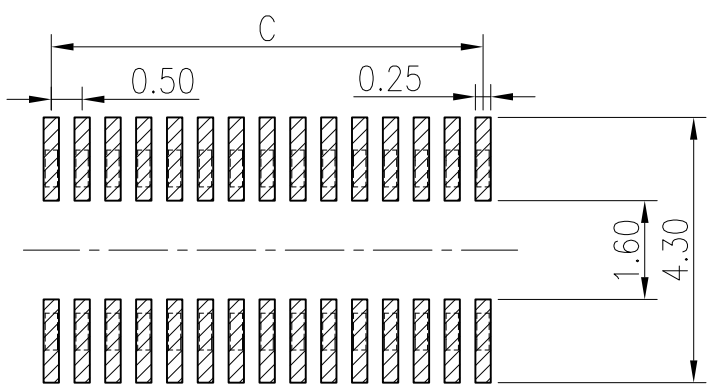
RECOMMENDED PCB PATTERN DIM. TOLERANCE : ±0.05
